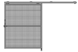
H8 - Double Panel W/O Legs - Slides Right
