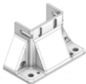
33-45903S-7 Mounting Foot- 3 Sided 45 X 90 105MM Tall 12MM Anchor Holes W/ Hardware
