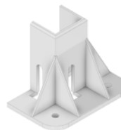
33-45453S-1 Mounting Foot 3 Sided 45 X45 11MM Anchor Holes W/ Hardware
